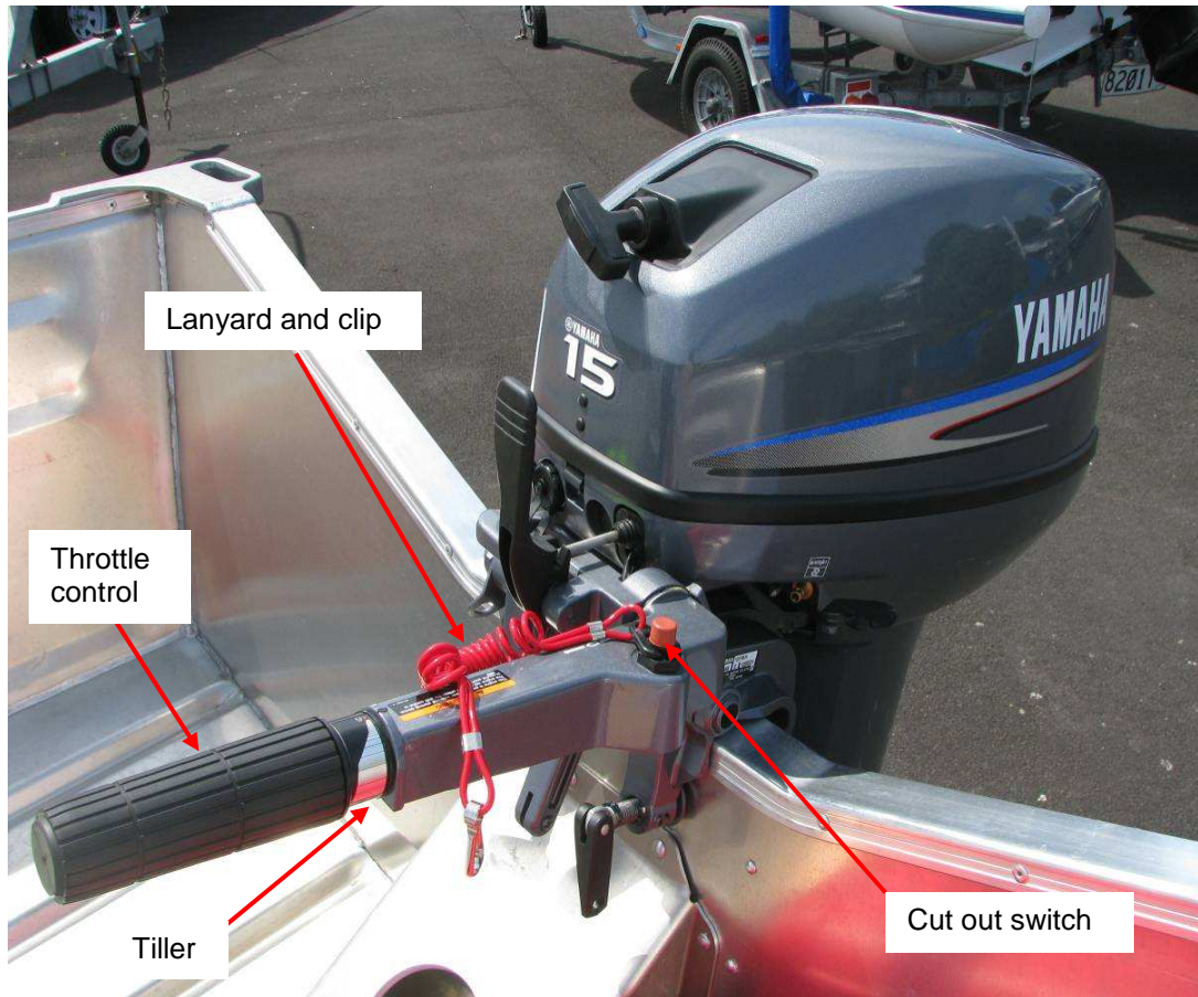
Figure 3 Similar vessel and motor showing lanyard arrangement
