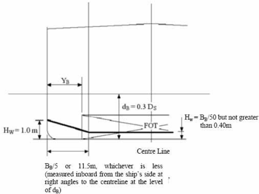
Figure 3 – Dimensions for calculation of the minimum oil outflow for the purpose of subrule (7)(e)(iii)(cc)
