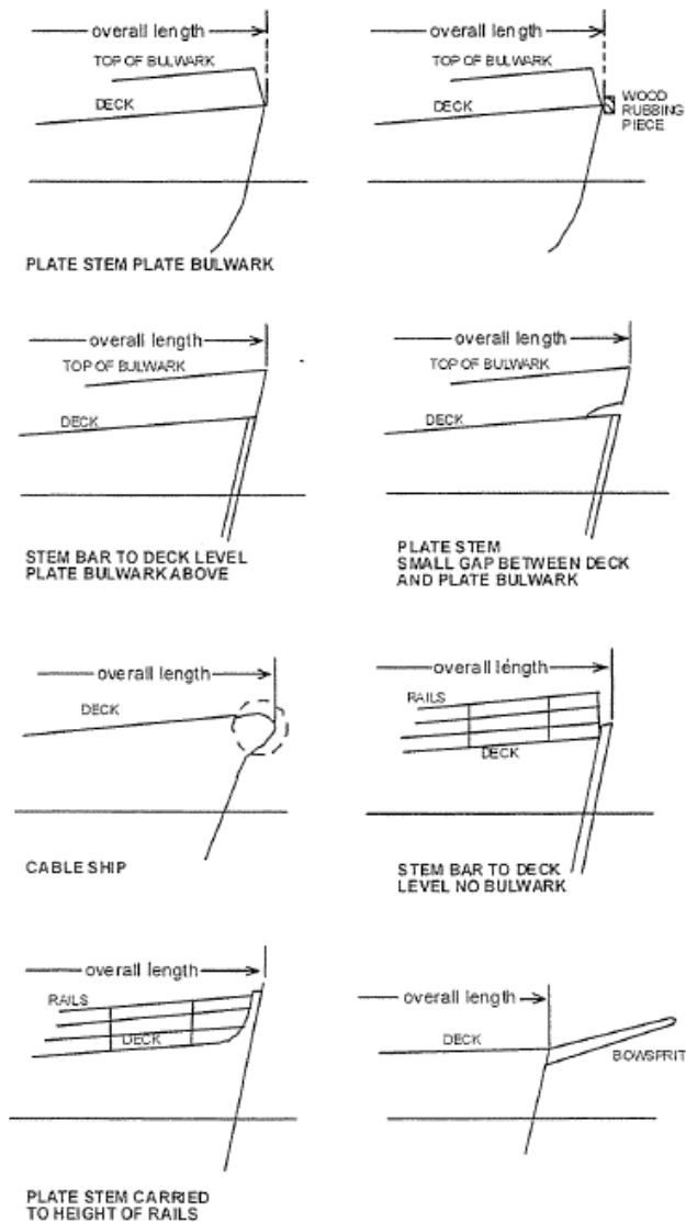
Types of stem
